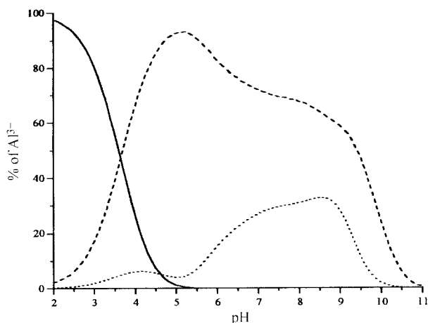
Fig. 3 Distribution profiles of free (solid line) and complexed fractions of aluminium in the presence of both HPH (dashed line) and \alpha -Alaha (dotted line). The \text{Al}^{3+}:\text{HPH}:\alpha\text{-Alaha} molar ratio was 1:8:8.
